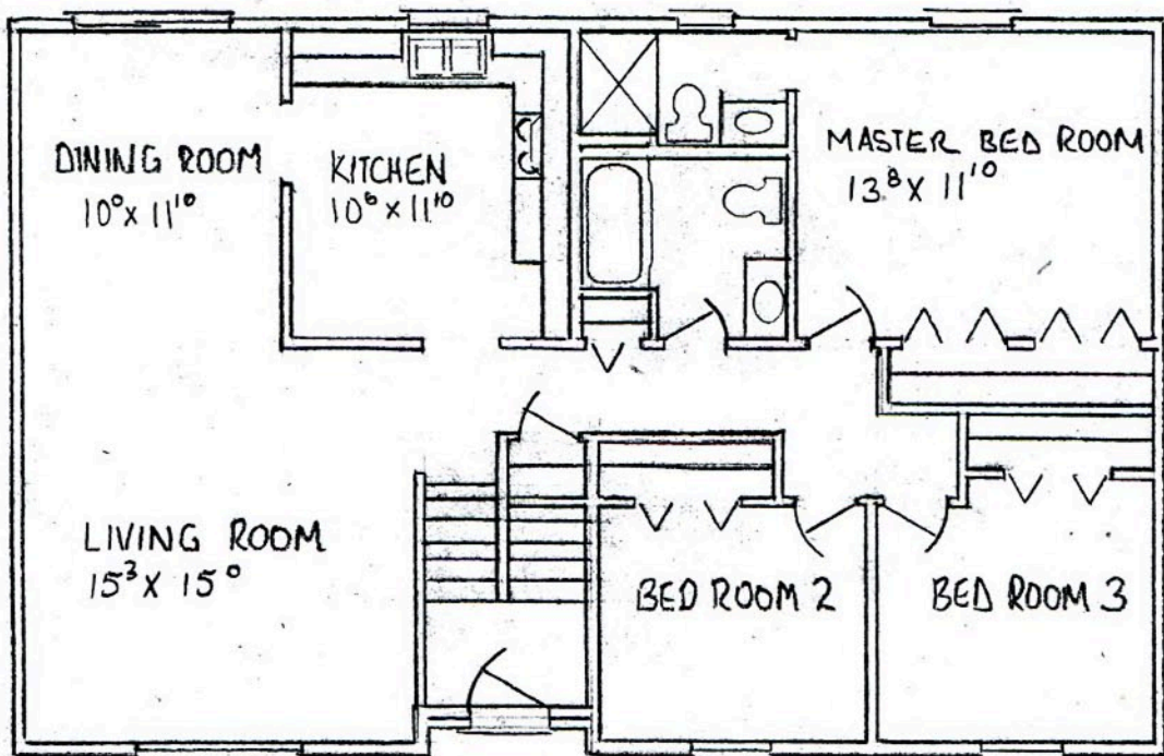
1st Floor - 1230 sq ft
